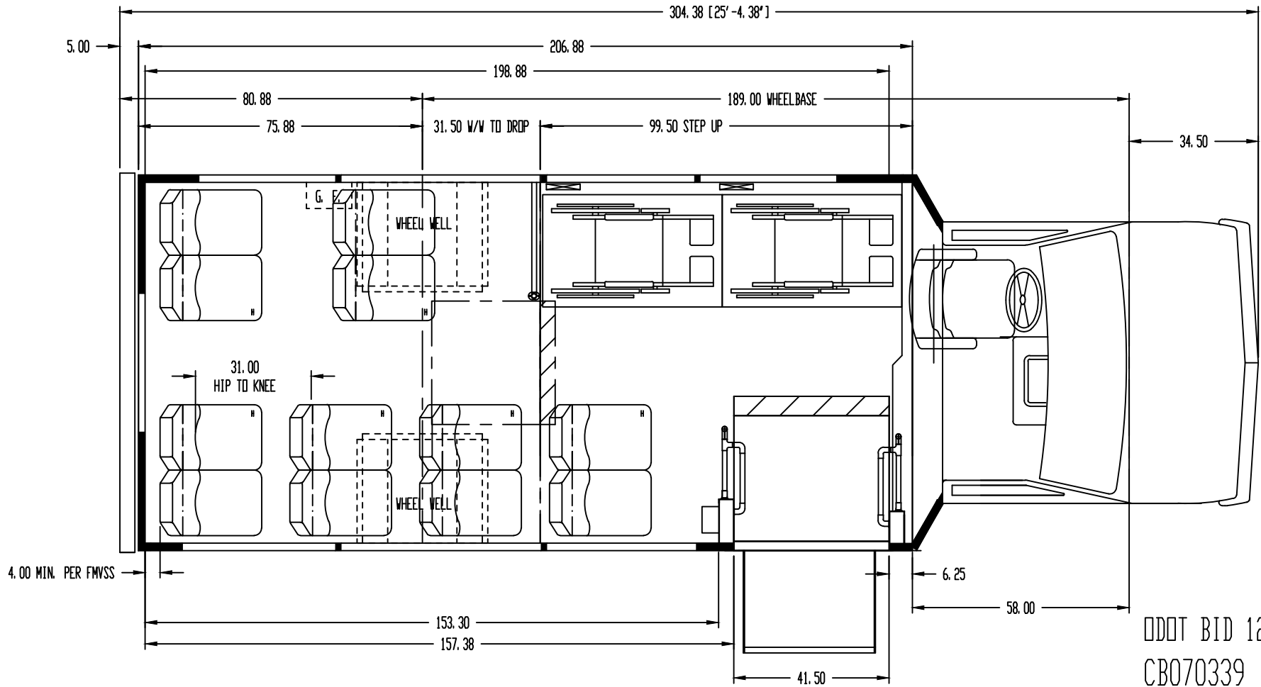
FLOORPLAN FORD LOW FLOOR-240 189.00' W/B
